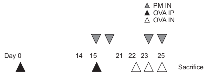
Supplementary Figure S1. Animal model design protocol. IN: intranasal treatment; IP: intraperitoneal treatment; OVA: ovalbumin; PM: particulate matter.
