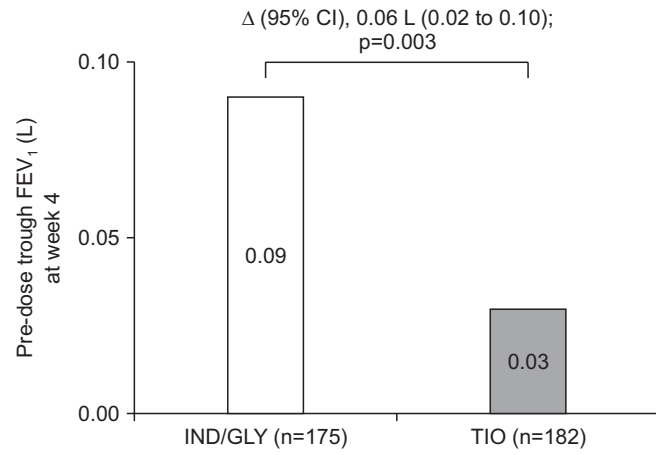
Supplementary Figure S1. Treatment difference between IND/GLY and TIO in pre-dose trough FEV 1 (L) at week 4 (FAS). Data are presented as least squares means. IND/GLY: indacaterol/glycopyrronium 110/50 µg once daily; TIO: tiotropium 18 µg once daily; FEV 1 : forced expiratory volume in 1 second; FAS: full analysis set; \Delta : least square means treatment difference; CI: confidence interval.
